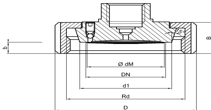
Conical nut connections PN 40 bar
