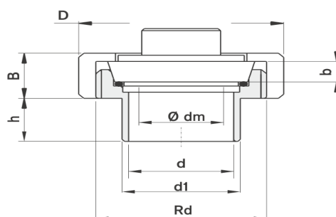
Conical unions with welding neck connections PN 40 bar
